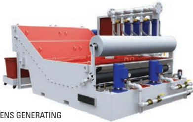
LENS GENERATING COOLANT FILTER
